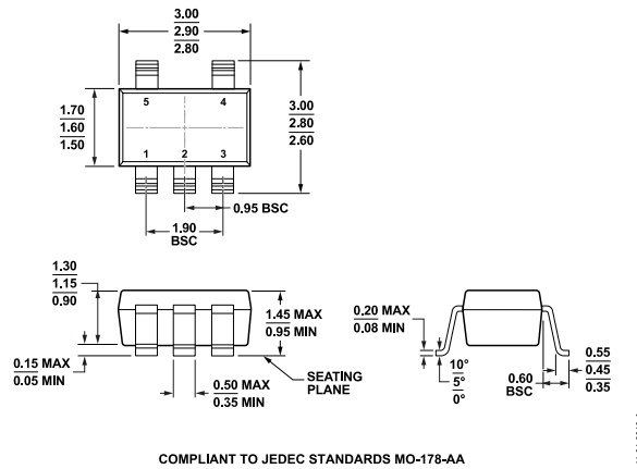
Figure 22. 5-Lead Small Outline Transistor Package [SOT-23] (RJ-5) Dimensions shown in millimeters
