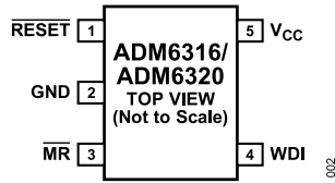
Figure 3. ADM6316/ADM6320 Pin Configuration
