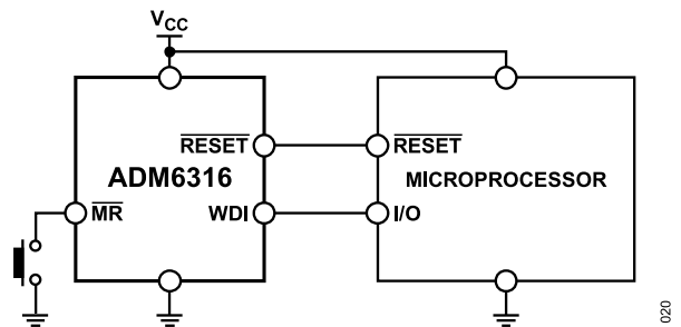
Figure 20. Typical Application Circuit
