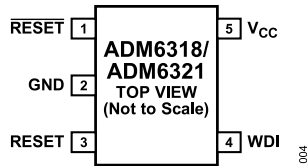
Figure 4. ADM6318/ADM6321 Pin Configuration
