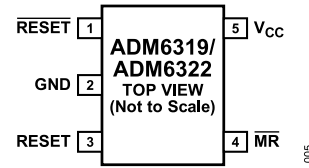
Figure 5. ADM6319/ADM6322 Pin Configuration
