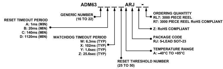
Figure 21. Ordering Code Structure (Modified Diagram)
