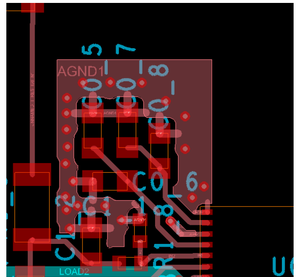
Figure 51. ADE1202 Pin 10 Close Up
