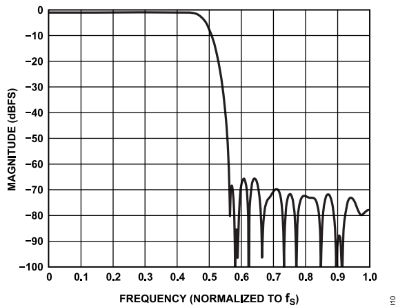
Figure 14. ADC Decimation Filter, 128× Oversampling, Normalized to f_s
