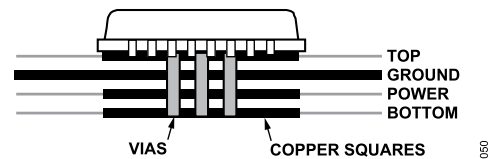
Figure 64. Exposed Pad Layout Example, Side View
