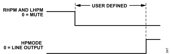
Figure 46. Headphone Output Power-Down Timing
