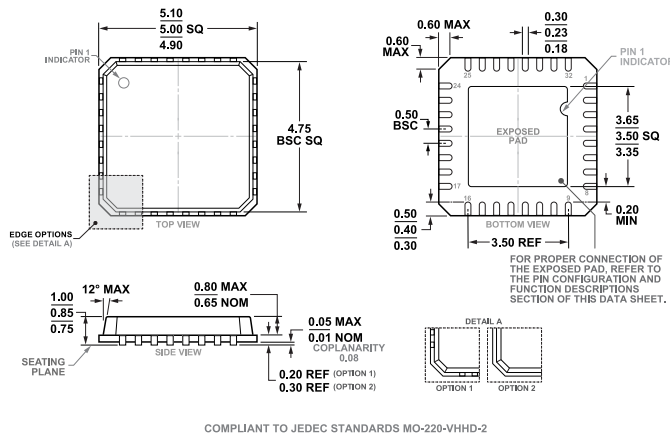
Figure 66. 32-Lead Lead Frame Chip Scale Package [LFCSP] 5 mm × 5 mm Body and 0.85 mm Package Height (CP-32-4) Dimensions shown in millimeters
