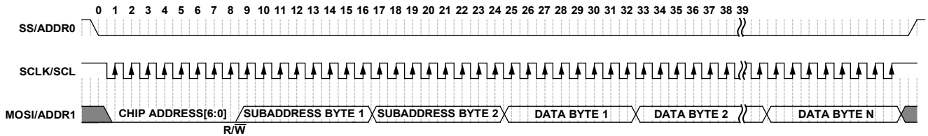
Figure 37. SPI Slave Write Clcking (Burst Write Mode, N Bytes)
