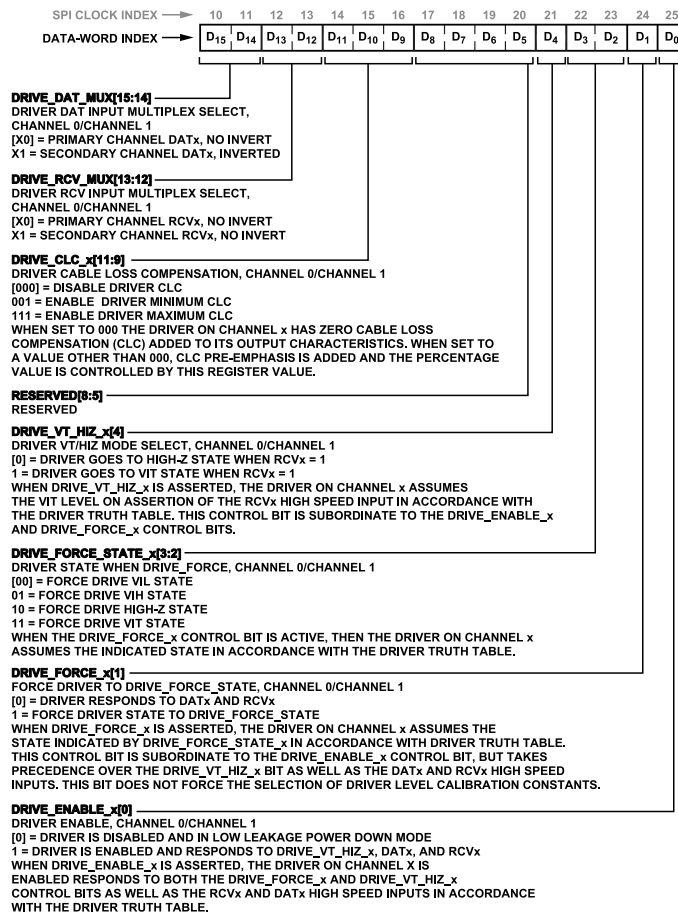
Figure 147. DRV Control Register (Address 0x19)
