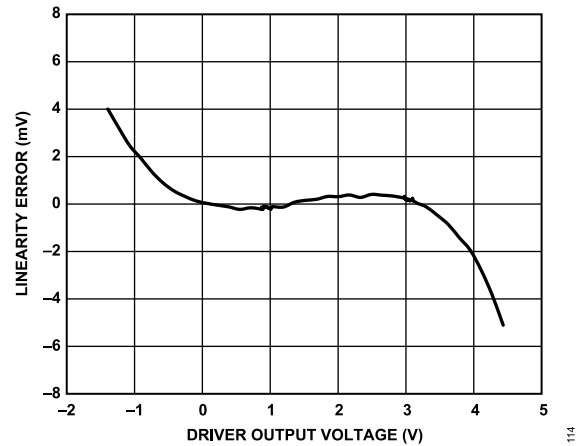
Figure 14. Driver VIH INL
