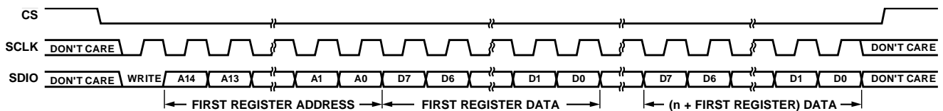
Figure 5. SPI Block Write
