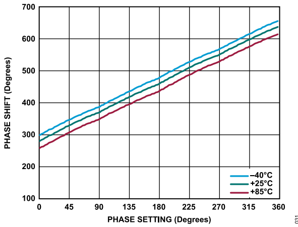
Figure 35. Phase Shift vs. Phase Setting over Temperature, Transmit Channel
