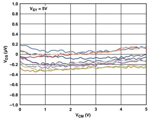
Figure 13. Input Offset Voltage vs. Common-Mode Voltage
