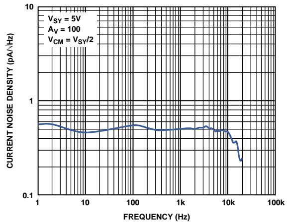
Figure 55. Current Noise Density vs. Frequency
