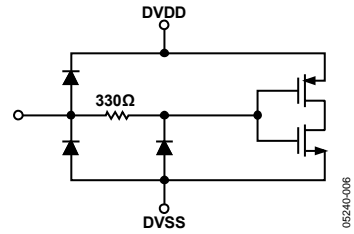
Figure 6. Digital Inputs
