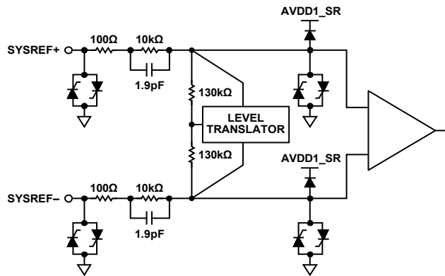
Figure 35. SYSREF± Inputs
