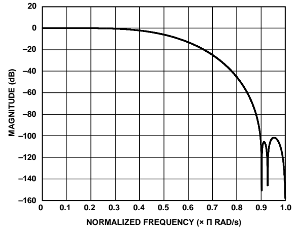
Figure 80. HB3 Filter Response
