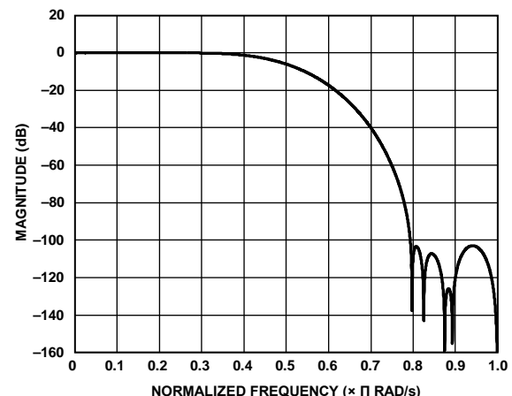
Figure 81. HB2 Filter Response
