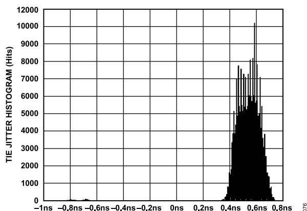
Figure 74. Time Interval Error (TIE) Jitter Histogram for LVDS Outputs in ANSI-644 Mode with Trace Lengths Greater than 24 Inches on Standard FR-4 Material, External 100 Ω Far-End Termination Only
