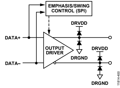
Figure 67. Digital Outputs
