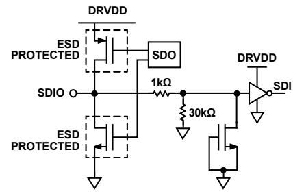
Figure 69. Equivalent SDIO Circuit
