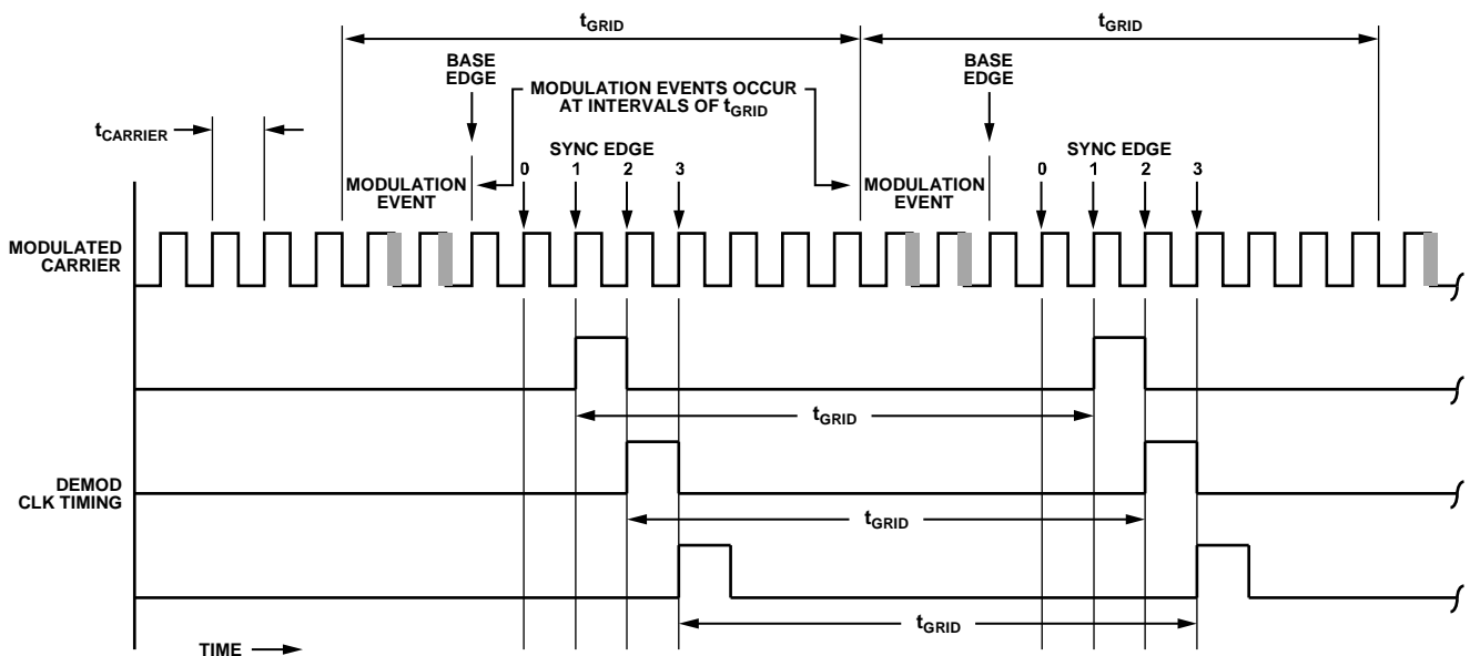
Figure 64. Demodulator Synchronization
