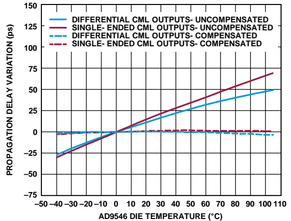
Figure 25. Propagation Delay Variation vs. AD9546 Die Temperature; CML Output Mode; 1.2 V CMOS Reference Input Mode; f_{SYS} = 2392 MHz; Internal Zero Delay (Hitless) Mode
