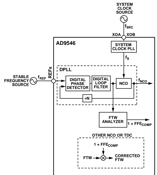
Figure 115. Closed-Loop Method
