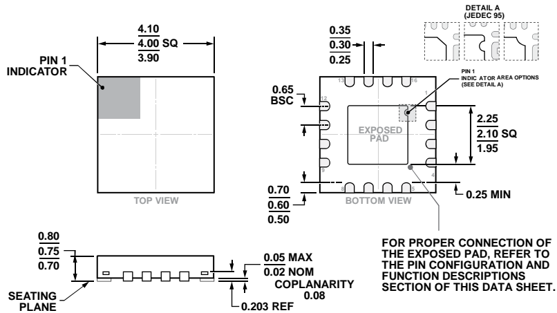
COMPLIANT TO JEDEC STANDARDS MO-220-WGGC. Figure 37. 16-Lead Lead Frame Chip Scale Package [LFCSP] 4 mm × 4 mm Body and 0.75 mm Package Height (CP-16-23) Dimensions shown in millimeters
