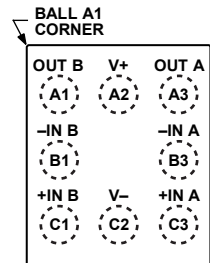
AD8506 TOP VIEW (BALL SIDE DOWN) Not to Scale
