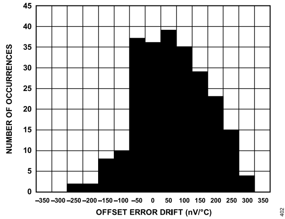
Figure 48. Offset Error Drift, DCLK = 32 MHz
