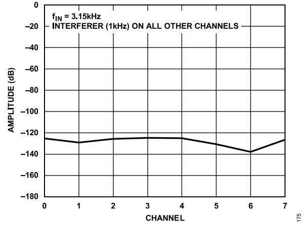
Figure 33. Crosstalk
