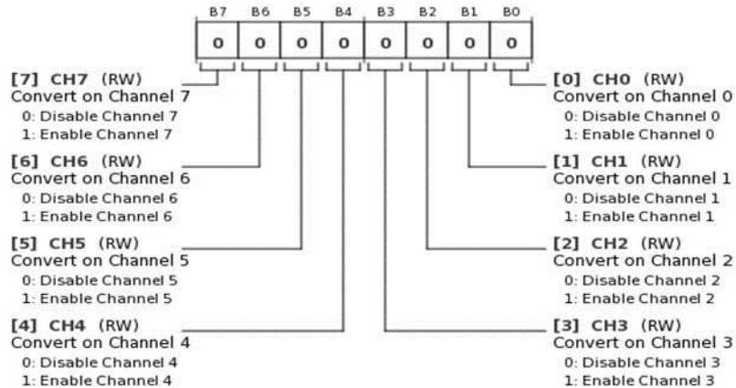
Figure 48. Channel Registers
