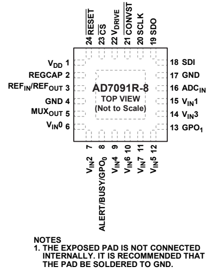
Figure 10. 8-Channel, 24-Lead LFCSP Pin Configuration
