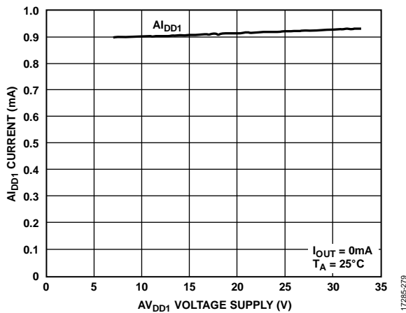
Figure 71. A_{I_{\text{DD1}}} Current vs. AV_{\text{DD1}} Voltage Supply
