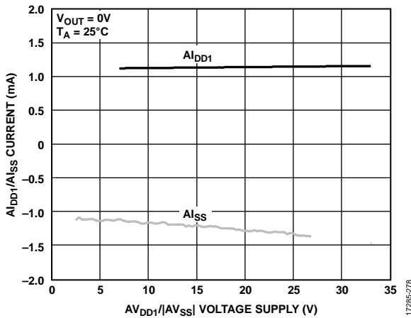
Figure 70. A_{I_{\text{DD1}}}/A_{I_{\text{SS}}} Current vs. AV_{\text{DD1}}/|AV_{\text{SS}}| Voltage Supply
