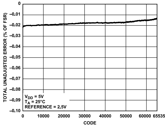
Figure 18. TUE vs. Code, AD5696
