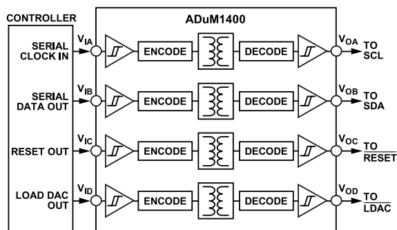
Figure 43. Isolated Interface
