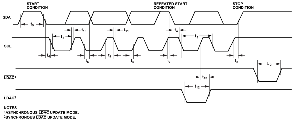
Figure 2. 2-Wire Serial Interface Timing Diagram
