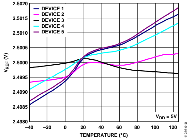
Figure 9. Internal Reference Voltage vs. Temperature (Grade A)
