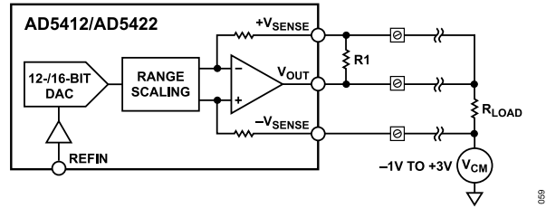
Figure 67. Voltage Output
