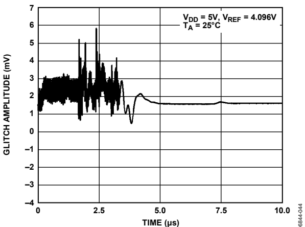
Figure 27. DAC-to-DAC Crosstalk
