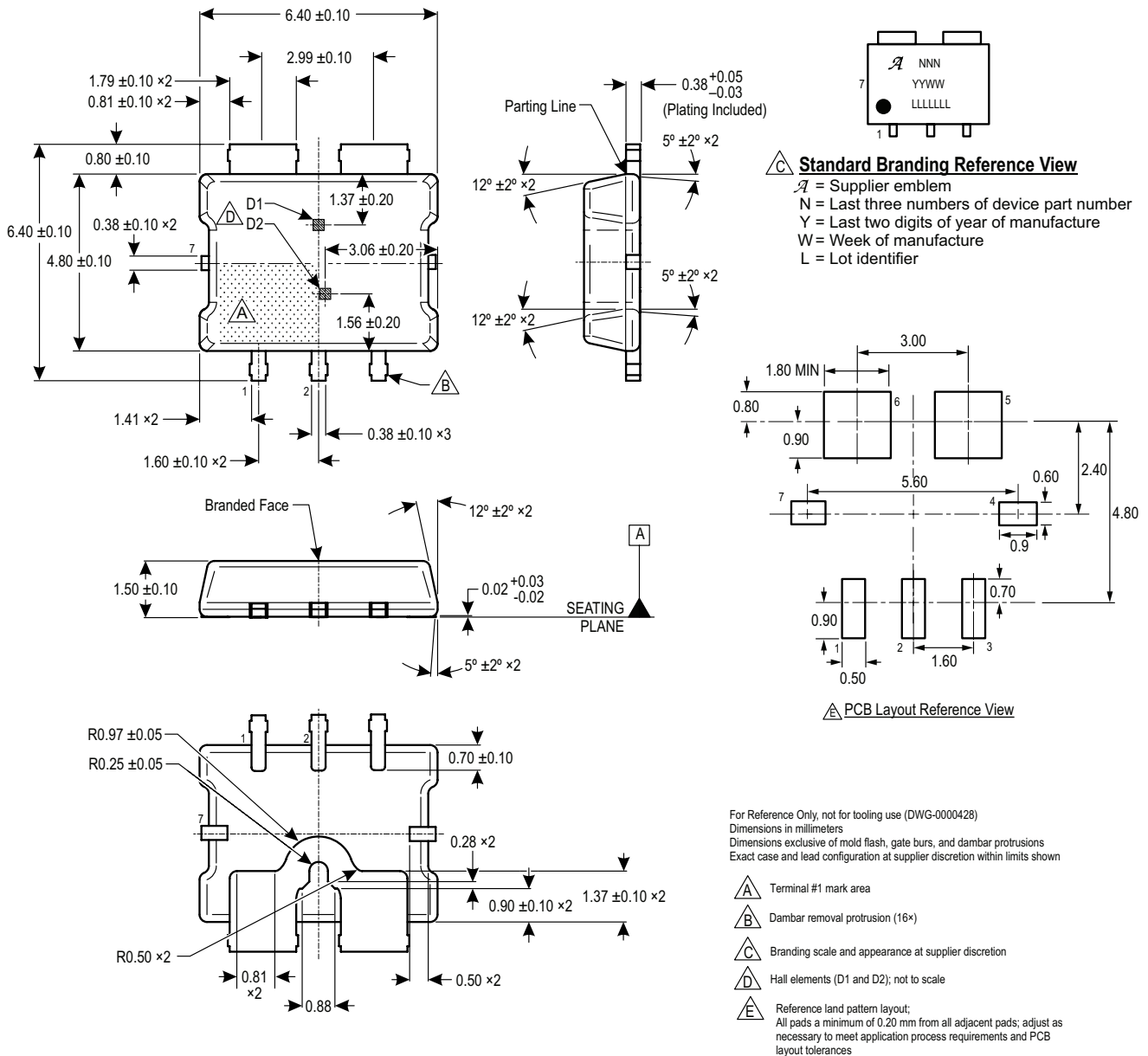
Package LR, 7-Pin PSOF Package
