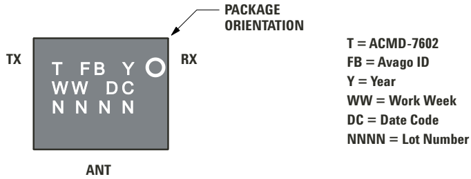
Figure 19. Package marking
