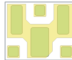
Figure 25. Solder stencil overlaid on AMCD-7602 bottom metal pattern
