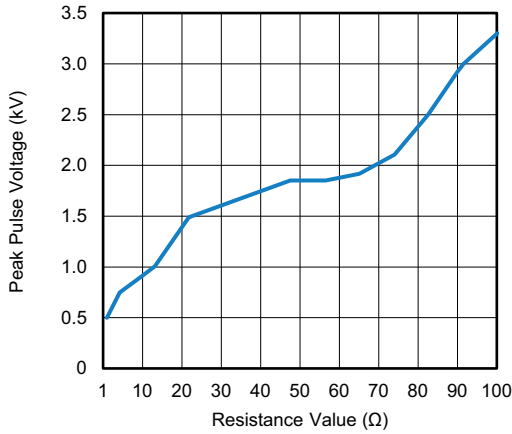
PEAK PULSE VOLTAGE LIMIT FOR AC01-CS (1.2 / 50 \mu s; 10 pulses at 30 s interval)
