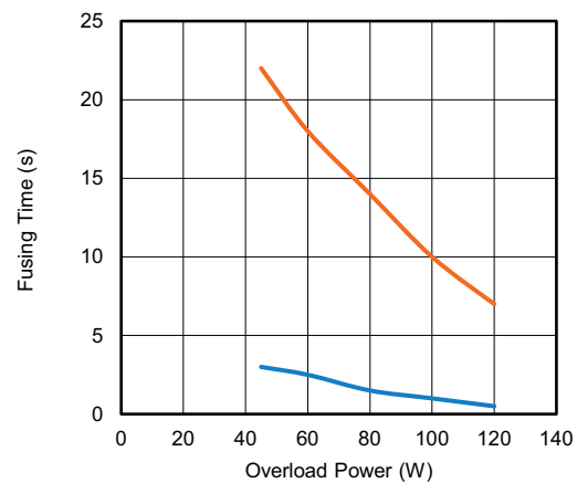
FUSING CHARACTERISTICS OF AC03-CS: 4.7 Ω ≤ R ≤ 100 Ω
