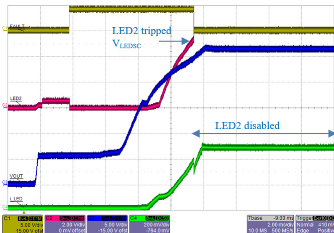
Figure 33: A80602 startup sequence when LED string#2 has a partial-short fault ( 6 \times \text{WLED} instead of 8). As soon as LED2 pin rises above V_{LESD} ( \sim 5\text{ V} ), the channel is disabled and FAULT = Low.
