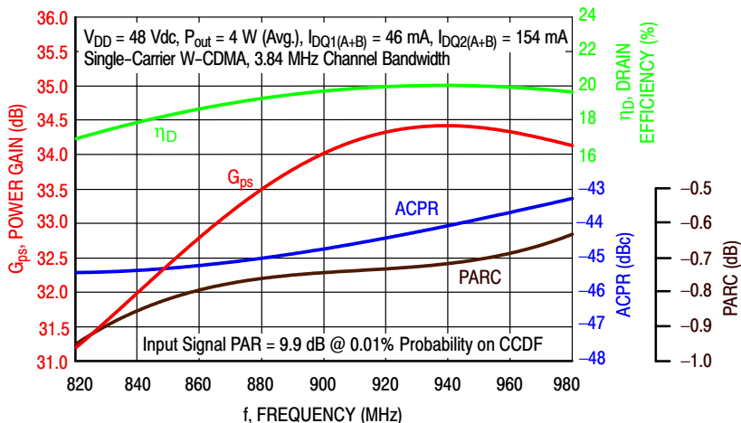
Figure 4. Single-Carrier Output Peak-to-Average Ratio Compression (PARC) Broadband Performance @ P_{out} = 4 \text{ Watts Avg.}
