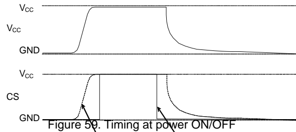
Figure 59. Timing at power ON/OFF (Bad example) CS pin is pulled up to Vcc. In this case, CS becomes "H" (active status), and EEPROM may have malfunction, mistake write owing to noise and the likes. Even when CS input is High-Z, the status becomes like this case, which please note. Bad example Good example (Good example) It is "L" at power ON/OFF. Set 10ms or higher to recharge at power OFF. When power is turned on without observing this condition, IC internal circuit may not be reset, which please note.
