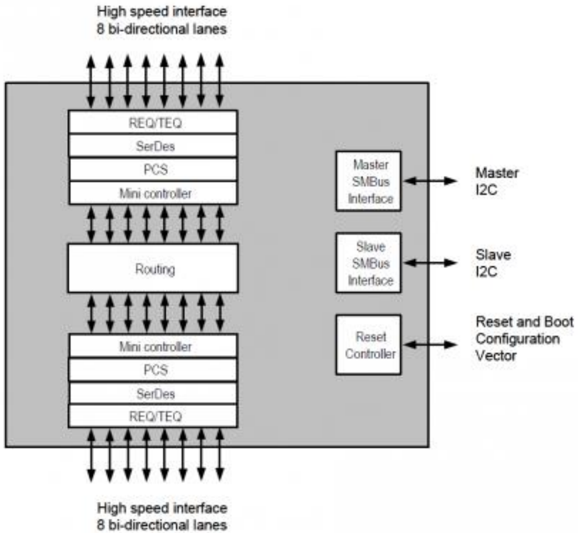
89HT0816AP - Block Diagram
