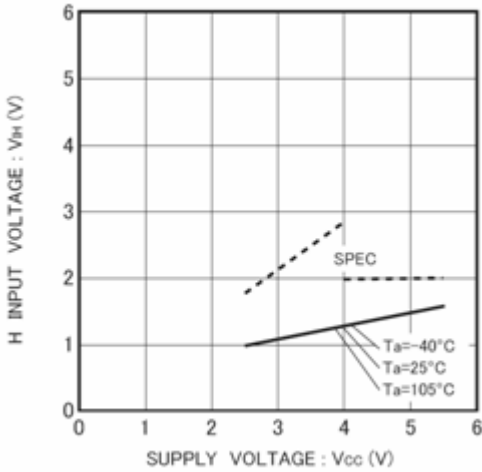
Figure 1. H input voltage VIH (CS, SK, DI)
