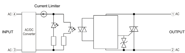
GN Series 20-265 V AC control
