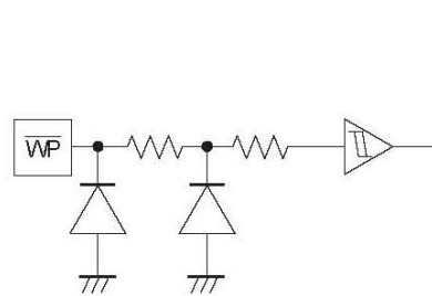
Figure 60. \overline{WP} input equivalent circuit
