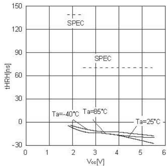
Figure 27. \overline{HOLD} release hold time t_{HRH}
