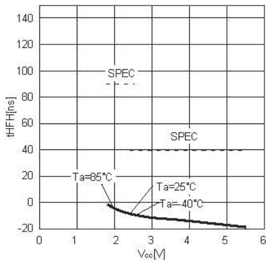
Figure 26. \overline{HOLD} setting hold time t_{HFH}
