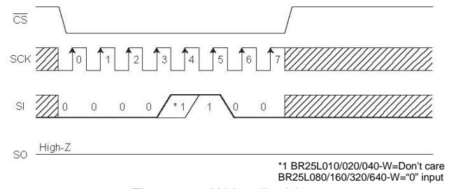
Figure 34. Write disable
