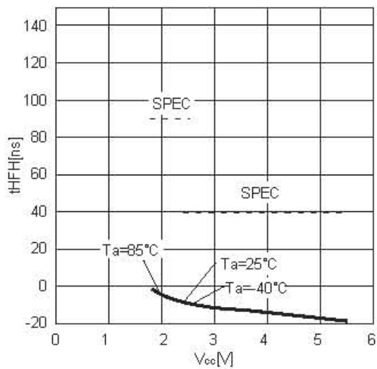
Figure 26. HOLD setting hold time t_{HFH}
