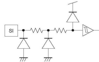
Figure 58. SI input equivalent circuit
