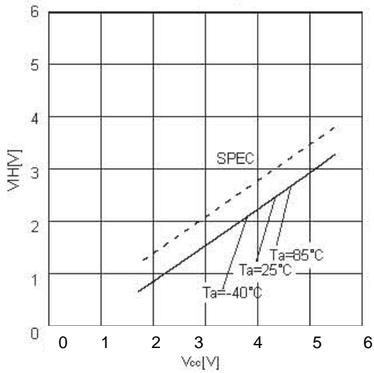
Figure 4. "H" input voltage VIH ( \overline{CS} , SCK, SI, \overline{HOLD} , \overline{WP} )
