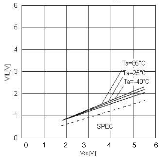
Figure 5. "L" input voltage VIL ( \overline{CS} , SCK, SI, \overline{HOLD} , \overline{WP} )
