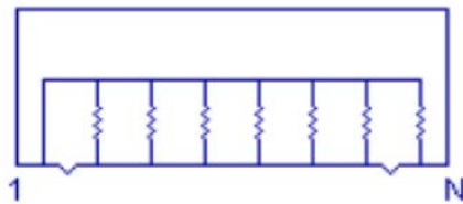
Bussed DRT [Schematic 1]
