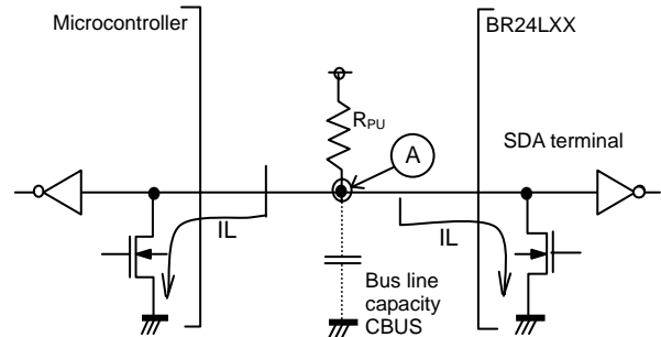
Figure 51. I/O circuit
