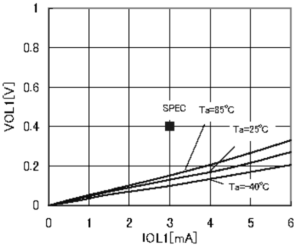
Figure 4. "L" Output Voltage V_{OL1} - I_{OL1} ( V_{CC}=2.5V )
