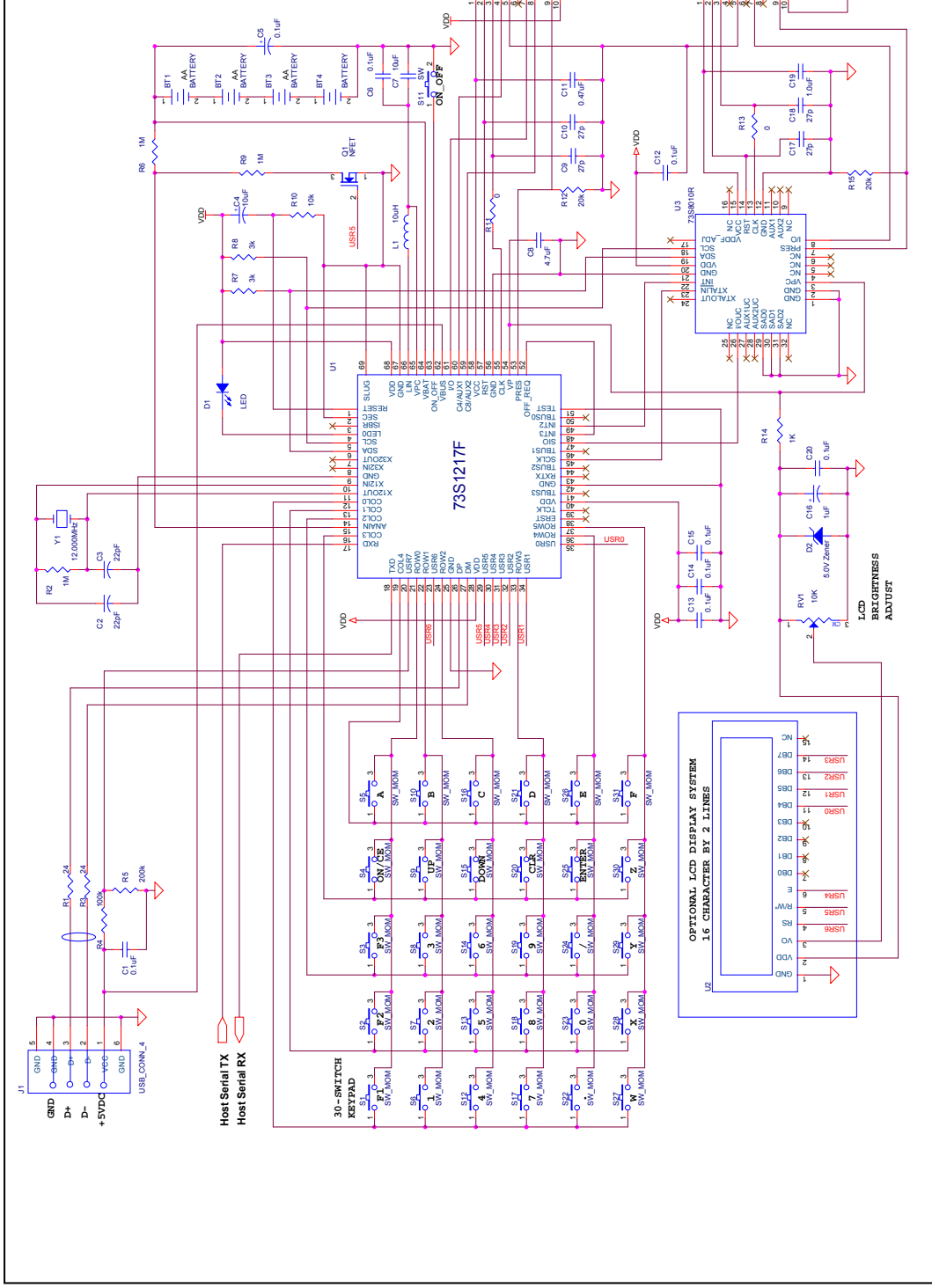
Figure 27: 73S1217F Typical Application Schematic (Handheld USB PINpad, with Combo USB-Bus and Self-power)
