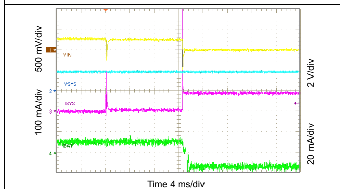
Figure 38. Entering DPPM Mode
