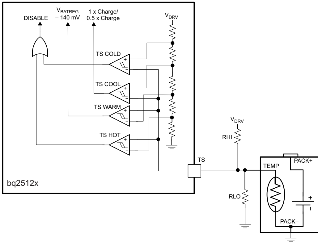
Figure 16. TS Circuit
