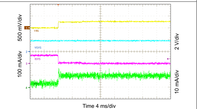
Figure 37. Power Supply Connected to V IN
