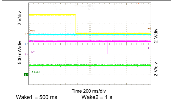
Figure 97. Show \overline{MR} Timing
