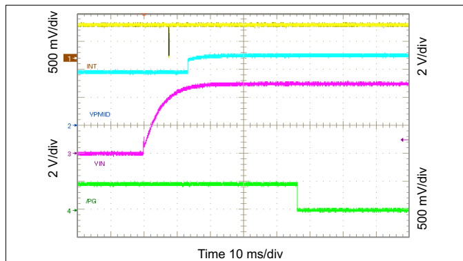
Figure 93. Show \overline{PG} and \overline{INT} Timing ( V_{IN} Insertion)
