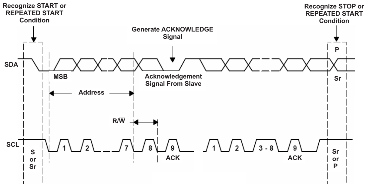
Figure 22. Bus Protocol
