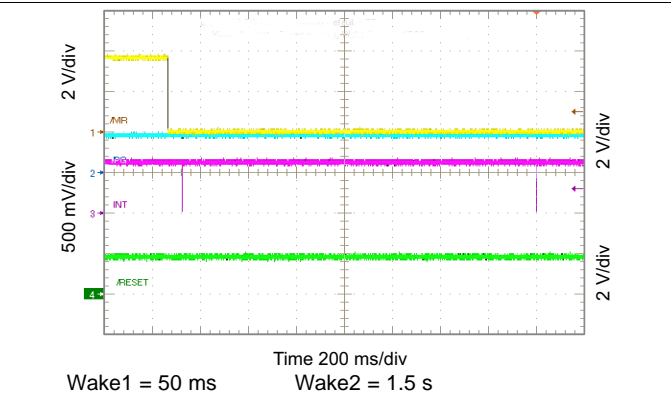
Figure 98. Show \overline{MR} Timing
