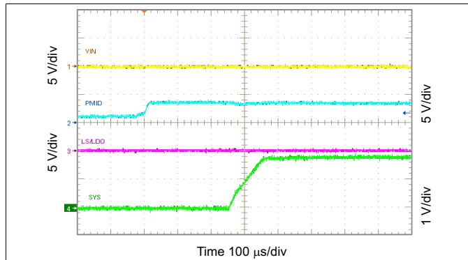
Figure 36. Battery Connected to V (BAT)
