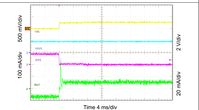
Figure 39. Exiting DPPM Mode
