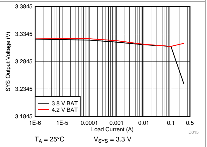
Figure 53. 3.3 V sys Load Regulation
