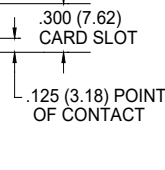
SINGLE ROW CONTACTS READ ONE SIDE OF DAUGHTER BOARD
