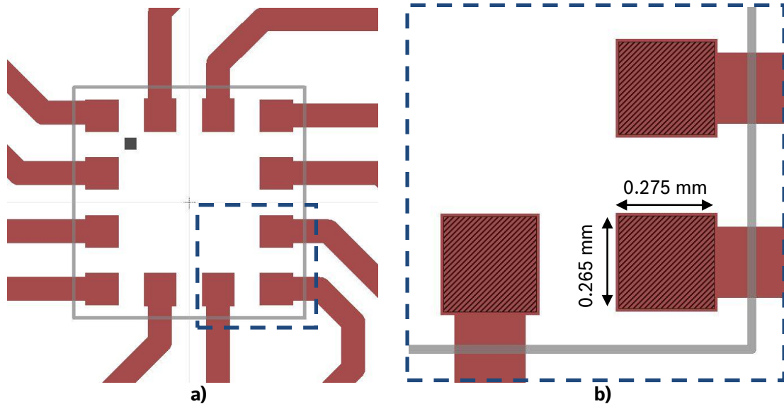
Figure 29: a) Landing patterns; b) solder paste pattern
