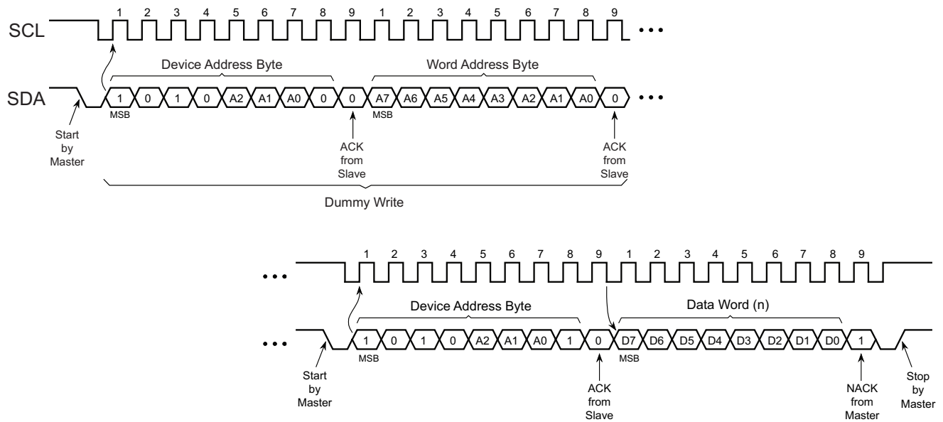
Figure 6-4. Random Read
