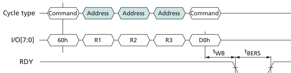
Figure 49: ERASE BLOCK (60h-D0h) Operation
