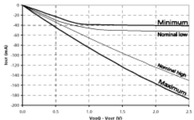
Figure 8: Pull-Up Characteristics
