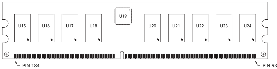
Figure 17: 184-Pin DIMM Dimensions – Very Low-Profile PCB
