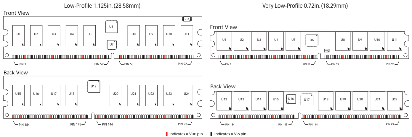
Figure 2: Pin Locations
