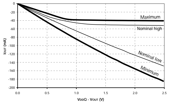
Figure 9: Pull-Up Characteristics
