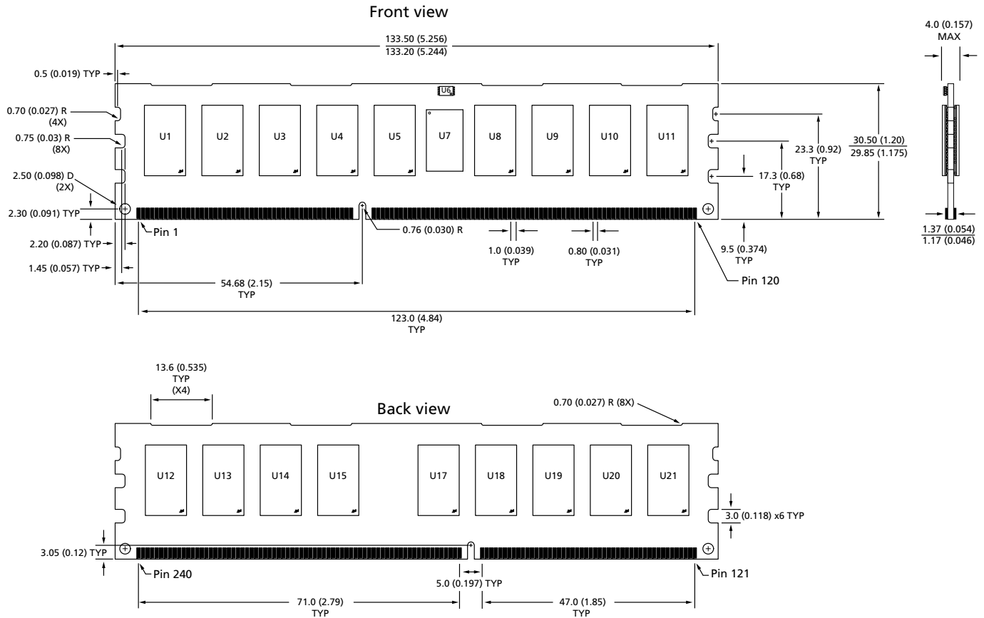
Figure 3: 240-Pin DDR3 RDIMM
