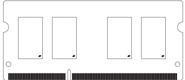
Figure 1: 204-Pin SODIMM (MO-268 R/C C)
